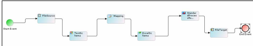
Figure 17.100: Connect Activities
