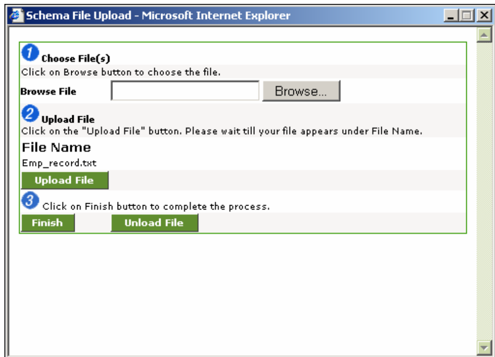
Figure 7.64: Uploaded File
