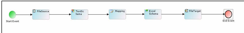
Figure 17.87: Scenario
