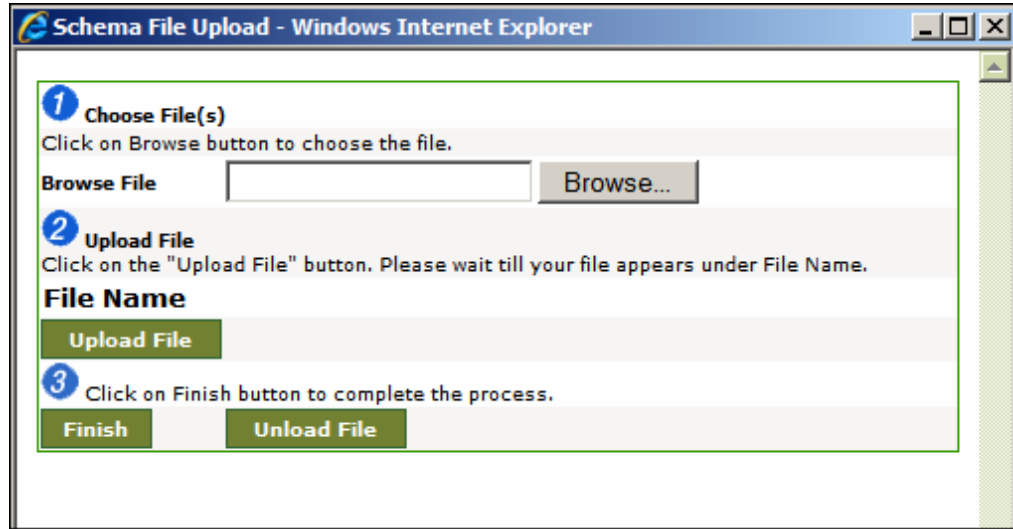
Figure 7.51: Upload file
