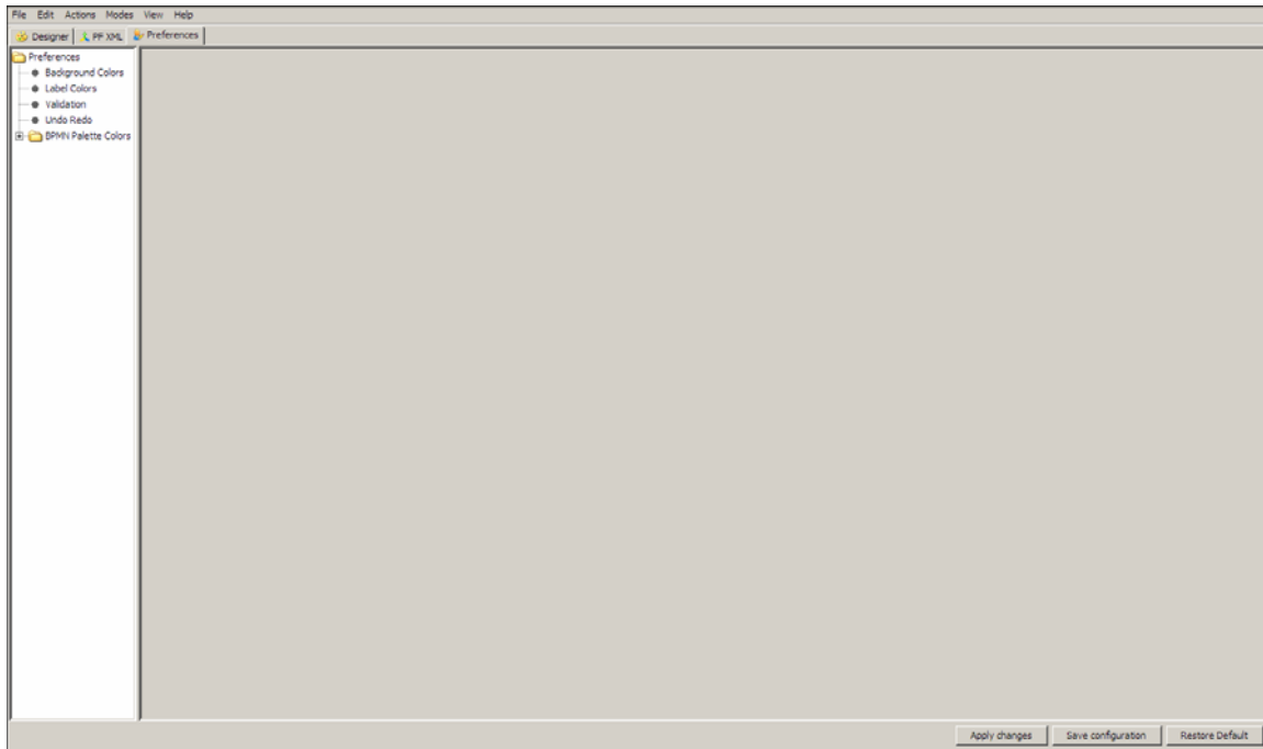
Figure 17.29: Changing Preferences
