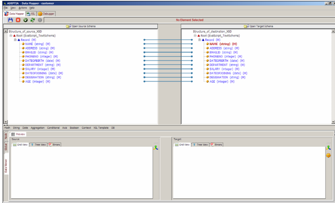
Figure 10.47: Data Viewer
