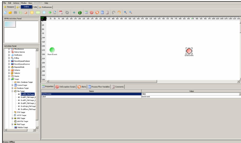
Figure 17.105: Changing Mode
