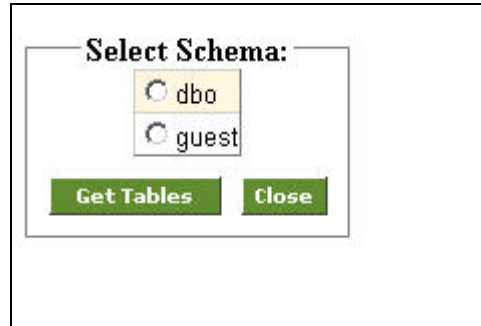
Figure 7.35: Select Schema
