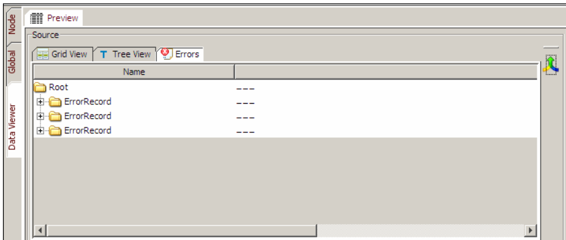
Figure 10.53: Error Record
