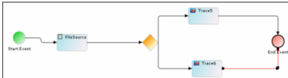
Figure 17.61: Connecting Elements
