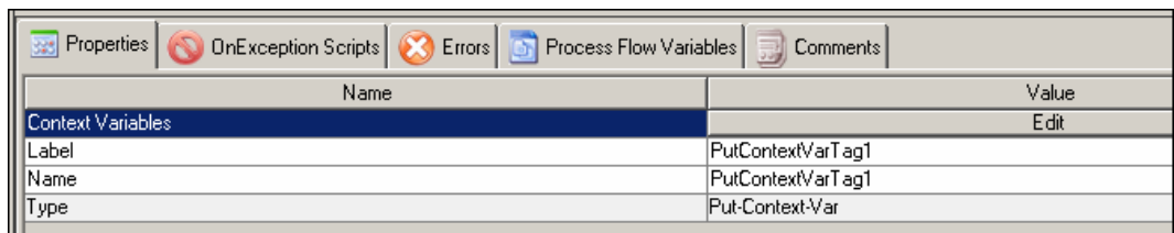
Figure 7.59: PutContextVar Properties
