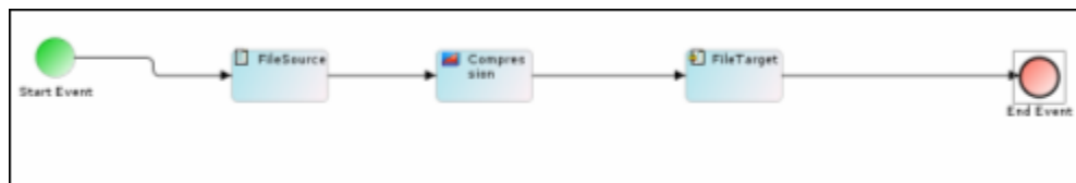
Figure 17.96: Connect Activities
