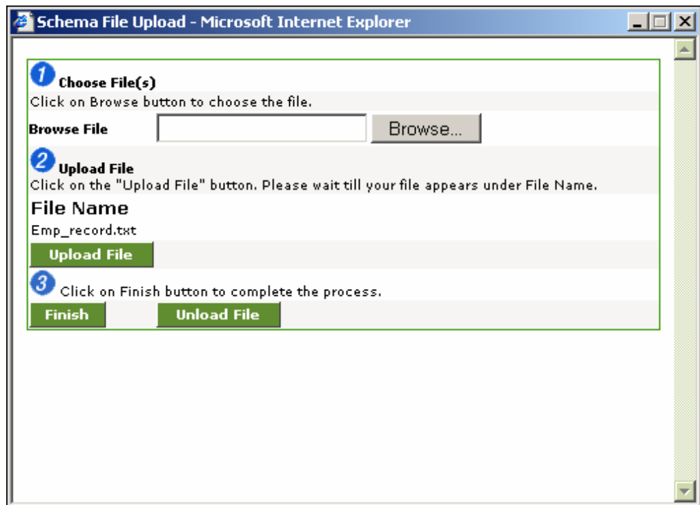
Figure 7.68: Uploaded File
