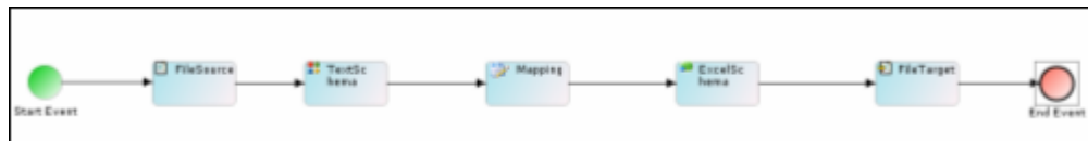
Figure 17.98: Scenario
