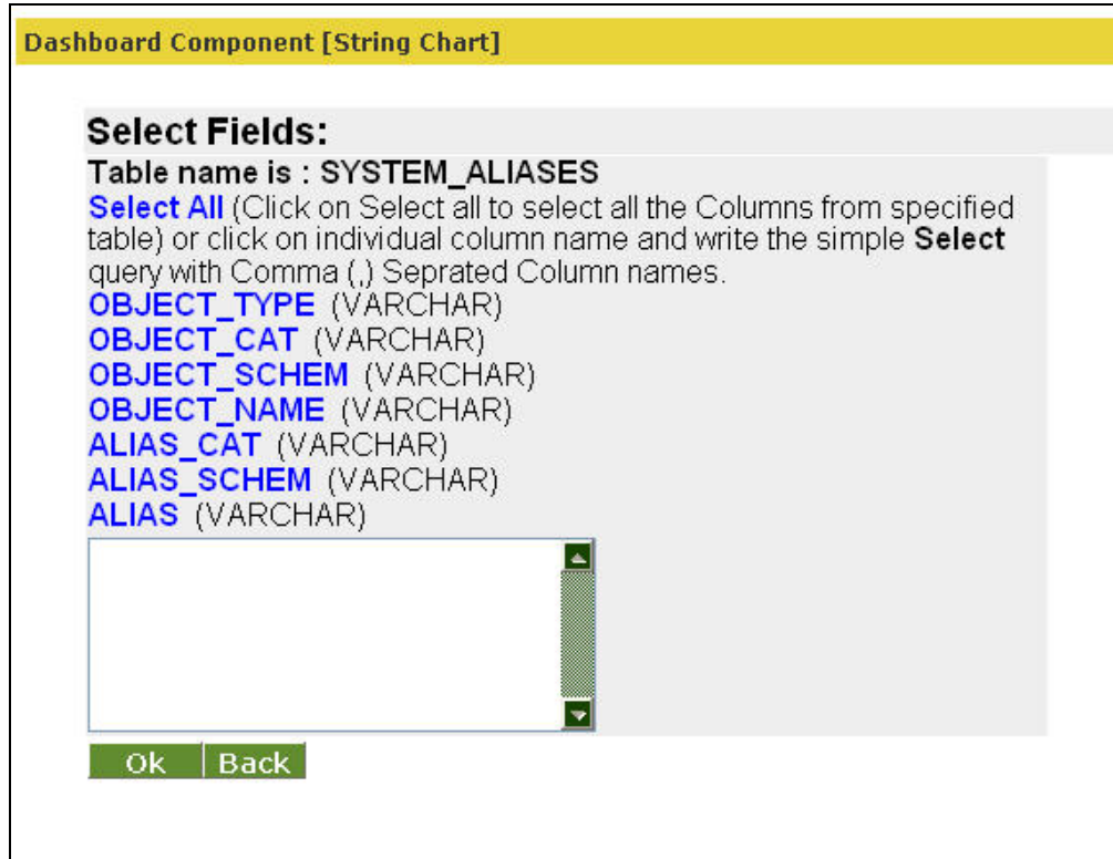
Figure 15.12: Select Fields
