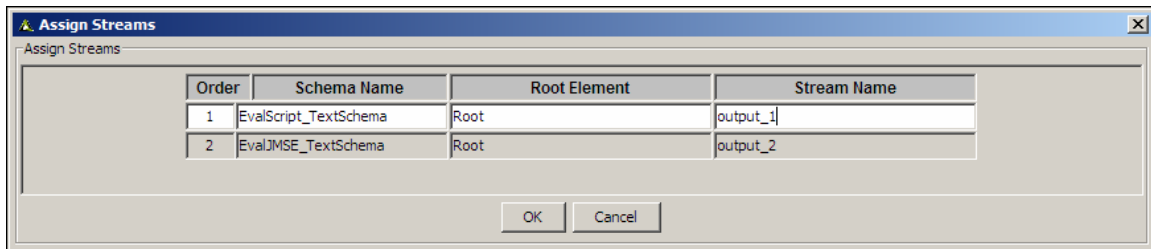
Figure 10.68: Assign Streams
