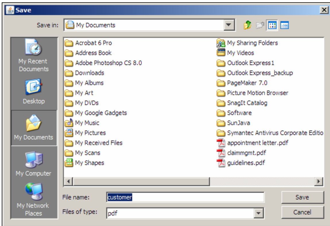
Figure 17.104: Save Box
