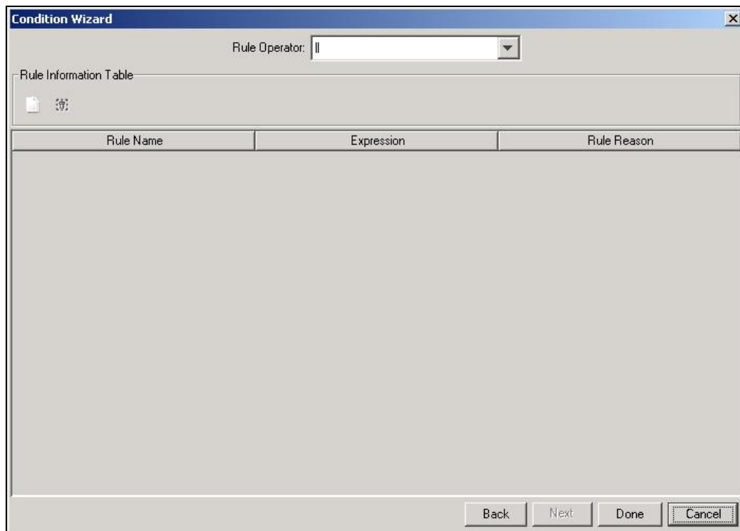
Figure 17.68: Condition Wizard
