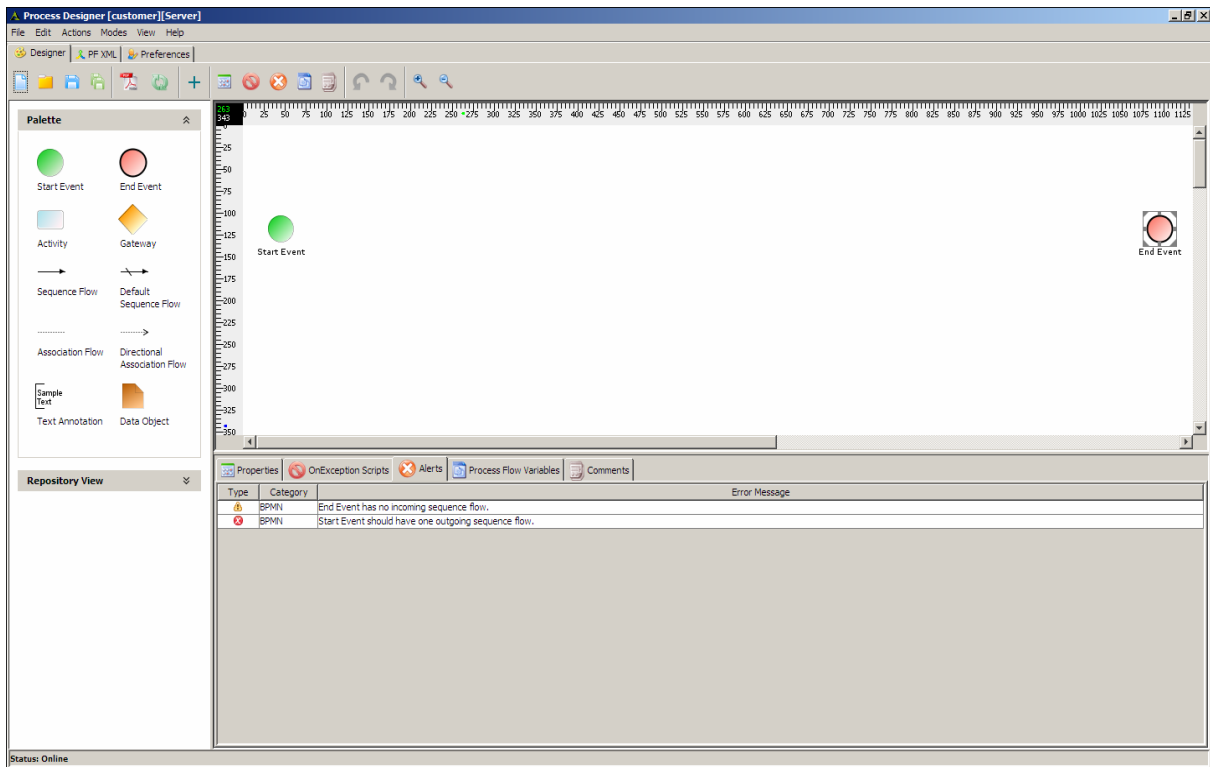
Figure 17.7: Process Designer
