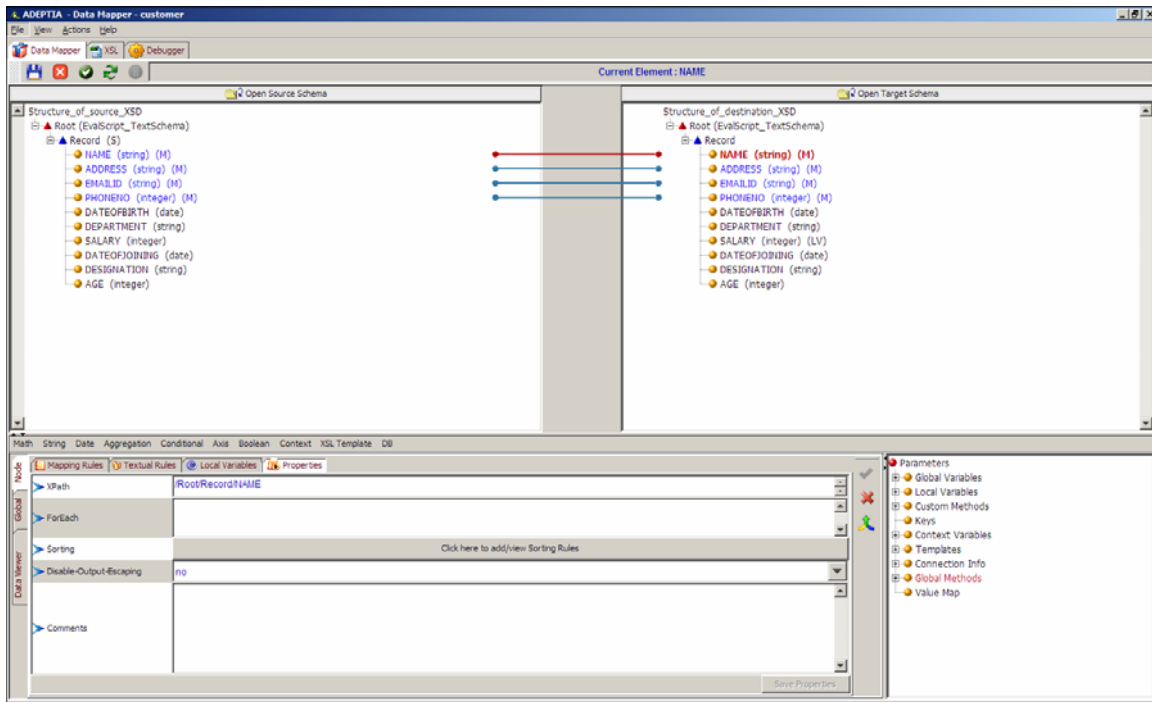
Figure 10.134: Properties Pane
