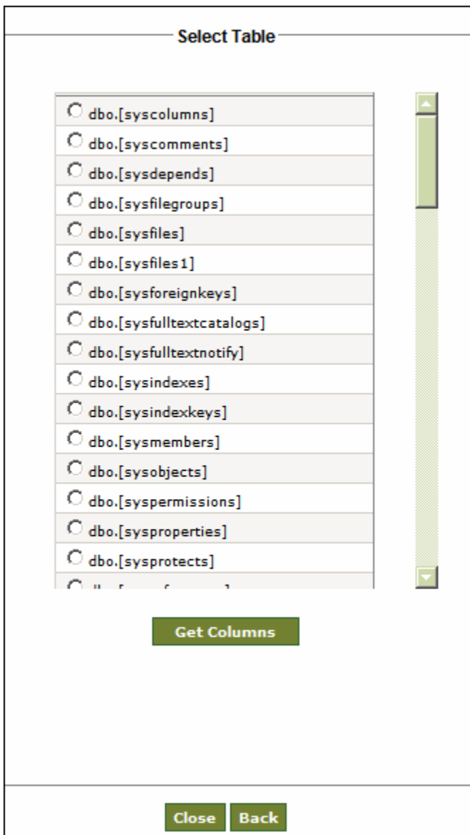
Figure 7.4: Select Tables
