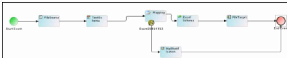
Figure 17.92: Connect Activities
