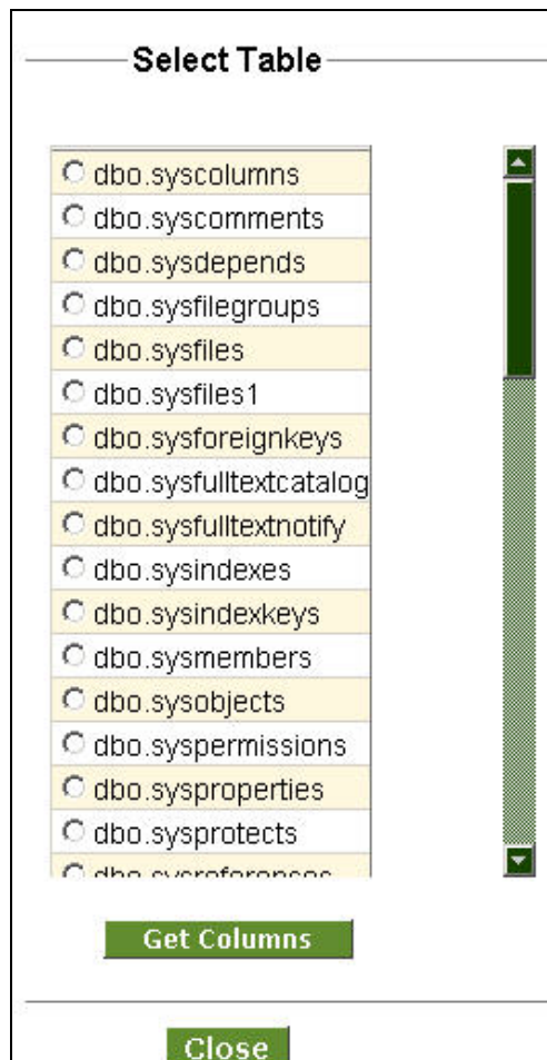
Figure 7.36: Select Tables
