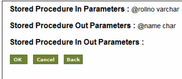
Figure 14.13: View Parameters
