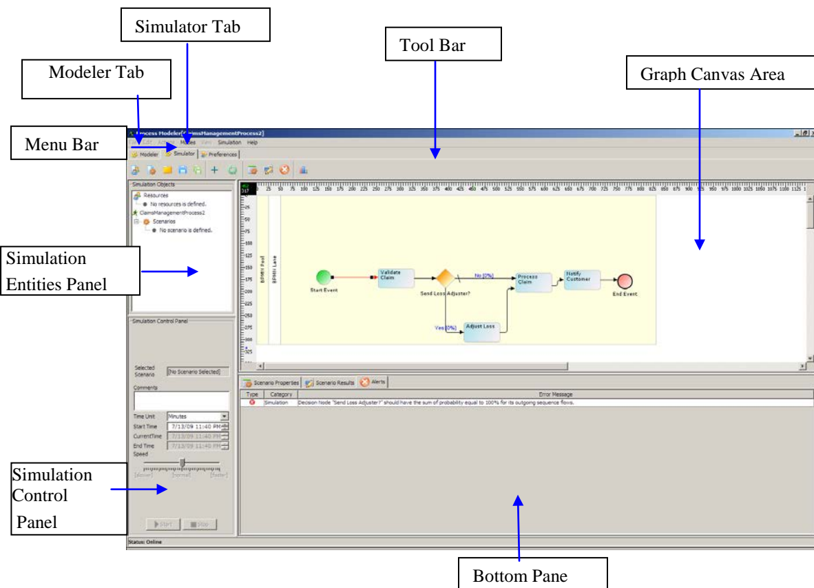
Figure 35: Process Simulation applet
